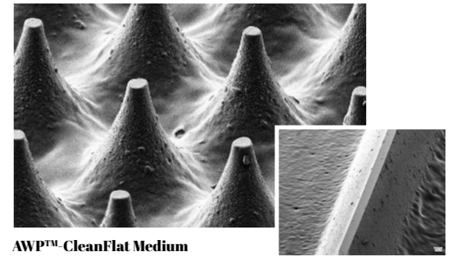
Crystal screen of AWP™-CleanFlat Medium
